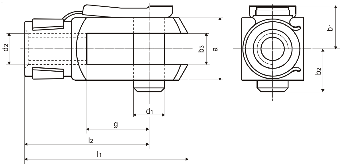
Type Z GAK 030 to Z GAK 140 A01
