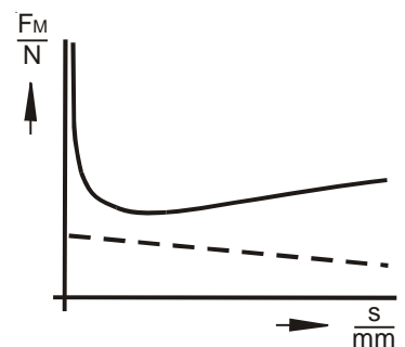
Fig. 2: Force characteristic
